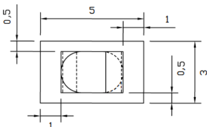
RECOMMENDED RESERVED AREA ON THE PCB (mm)
