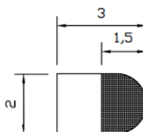
RECOMMENDED PAD FOR THE PCB (mm)
